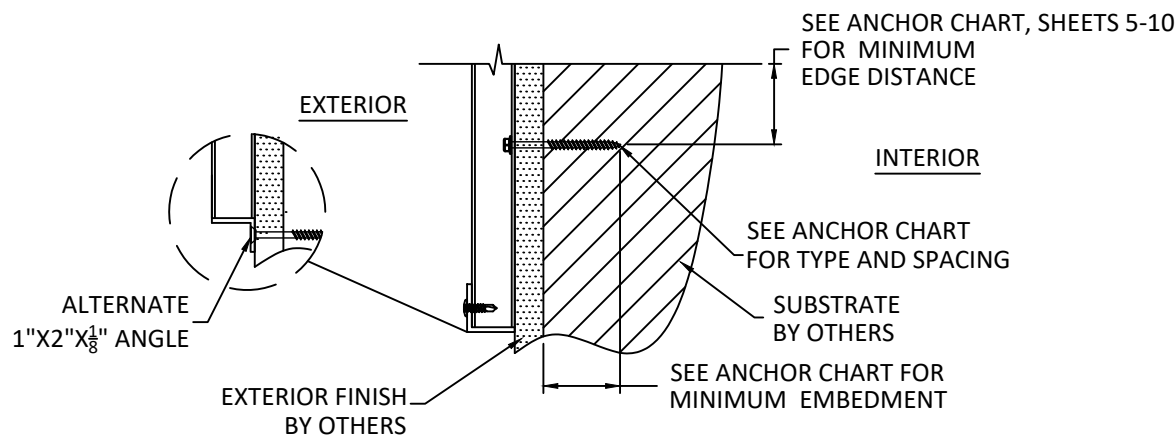
B 4 VERTICAL SECTION WALL MOUNT SEE CHARTS ON SHEETS 5-10 FOR DETAILS
