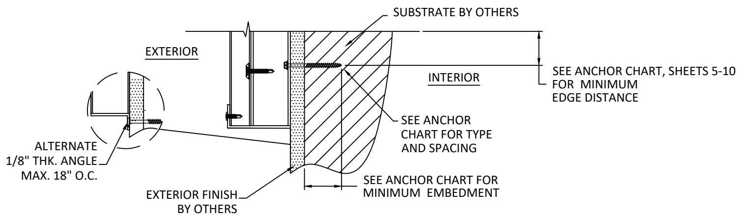
D 4 VERTICAL SECTION BUILT-OUT SEE CHARTS ON SHEETS 5-10 FOR DETAILS
