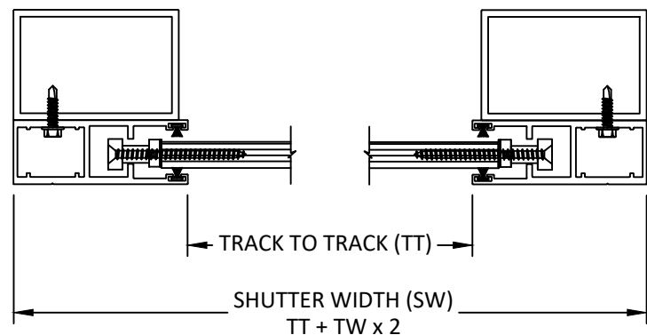
C 3 CROSS SECTION DETAIL MOUNT TYPE 3 WALL MOUNT
