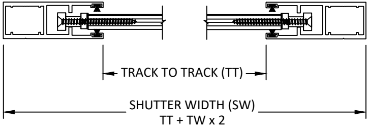
A 3 CROSS SECTION DETAIL MOUNT TYPE 1 BUILD OUT MOUNT
