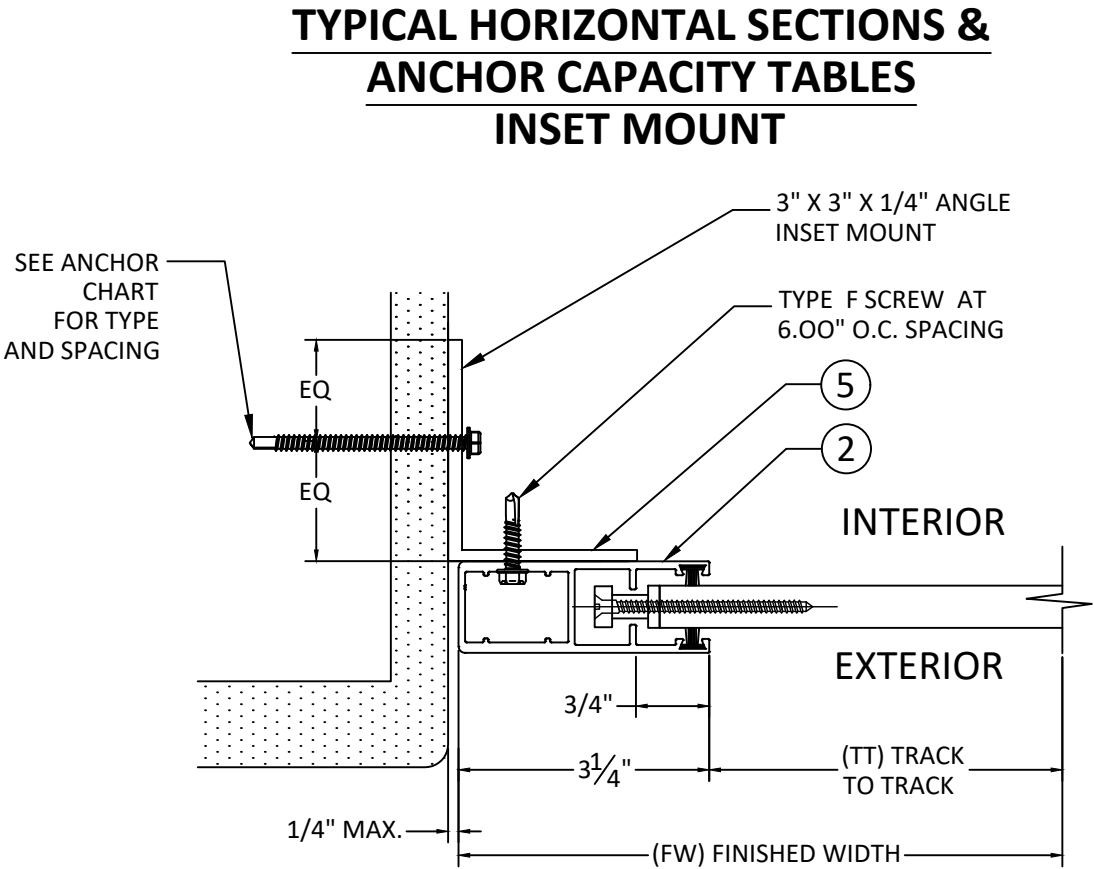
C 9 HORIZONTAL SECTION MOUNT TYPE 3 INSET MOUNT
