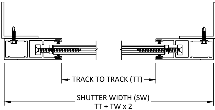
B 3 CROSS SECTION DETAIL MOUNT TYPE 2 INSET MOUNT
