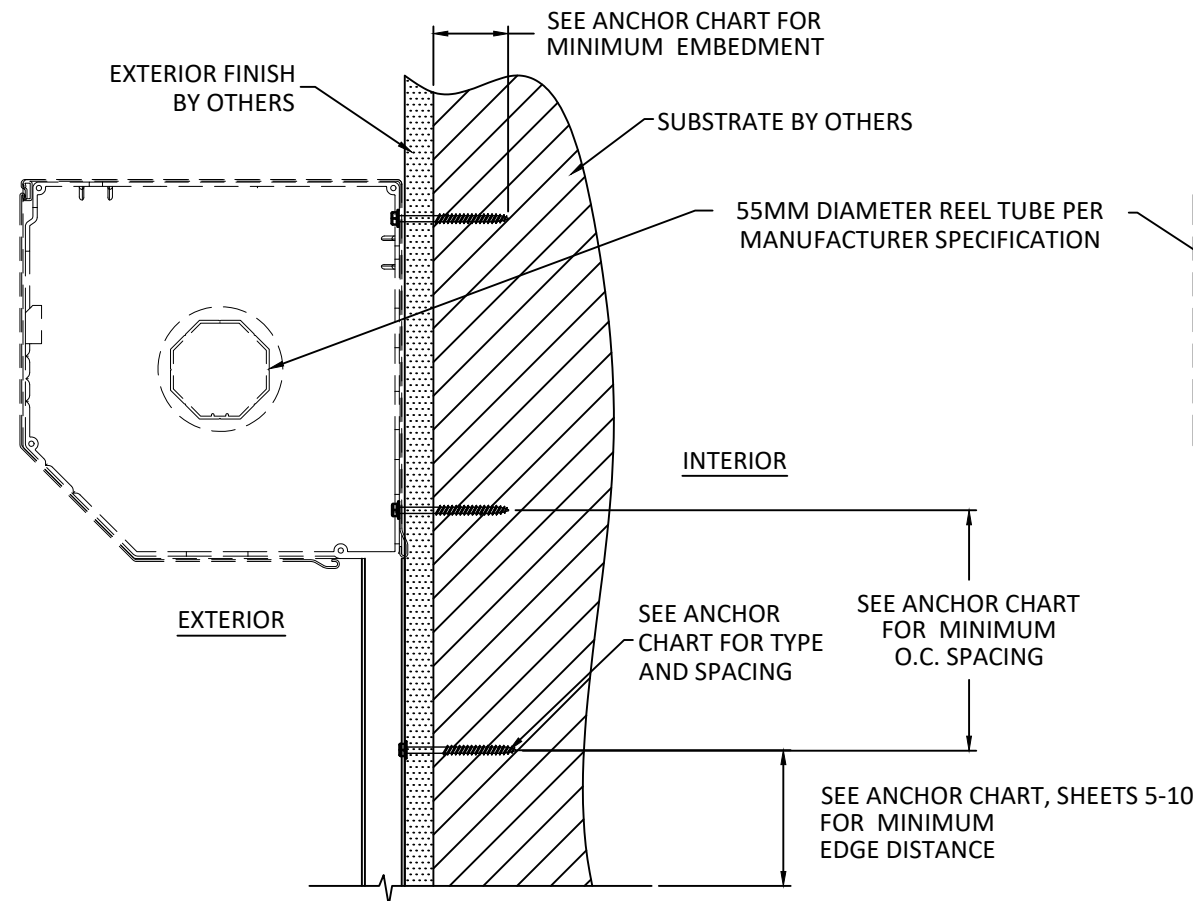
A 4 VERTICAL SECTION WALL MOUNT SEE CHARTS ON SHEETS 5-10 FOR DETAILS
