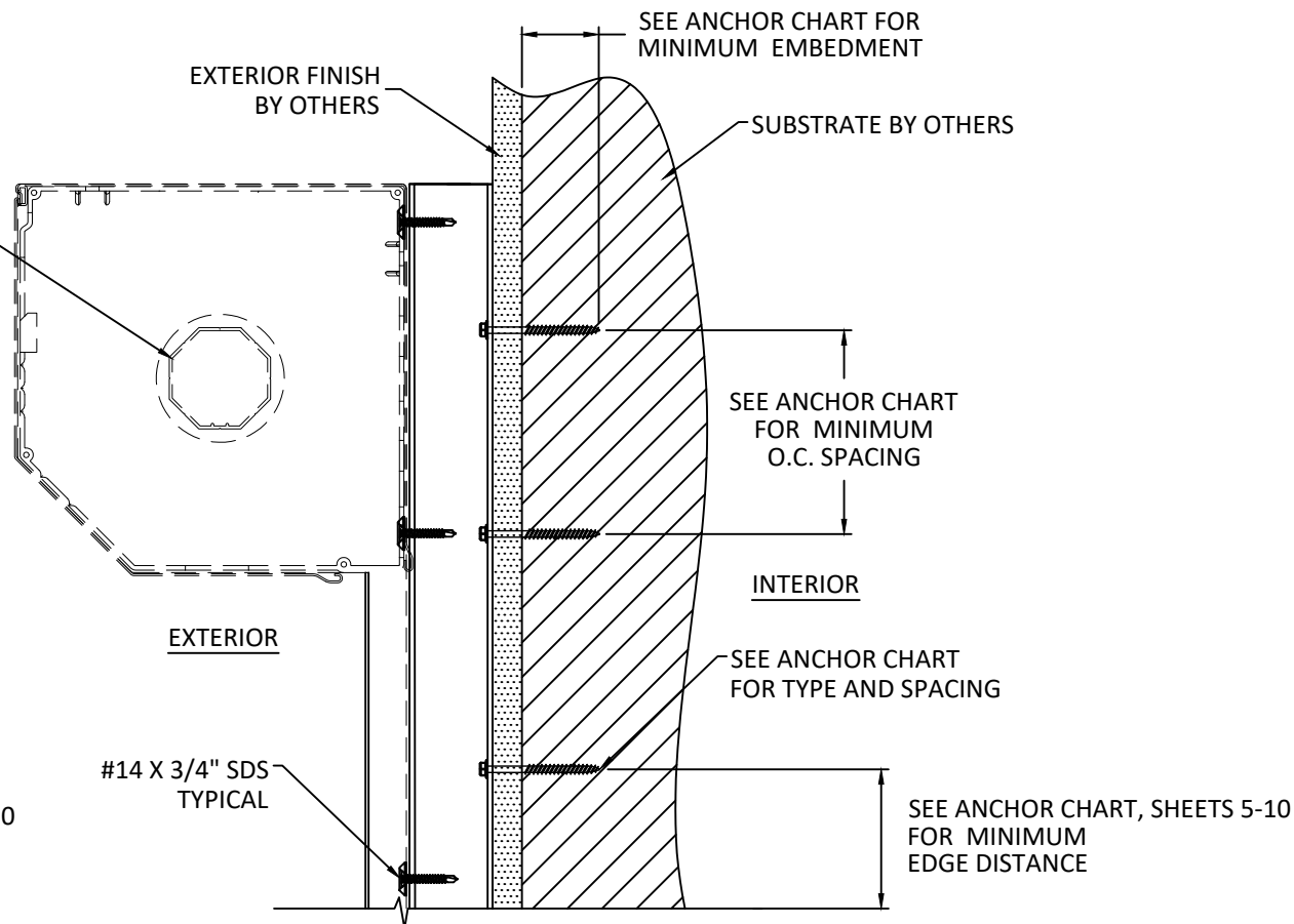
C 4 VERTICAL SECTION BUILT-OUT SEE CHARTS ON SHEETS 5-10 FOR DETAILS
